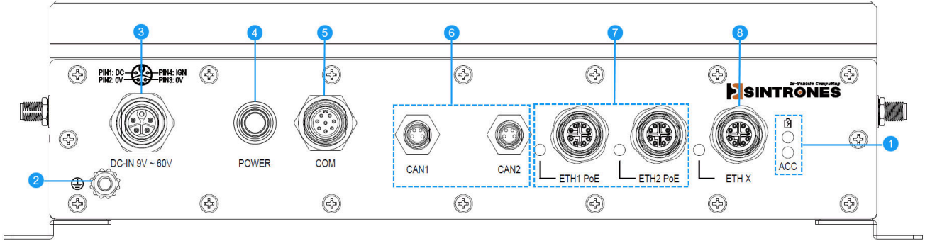
Figure 3-1 Front Panel of IBOX-650P-IP66
