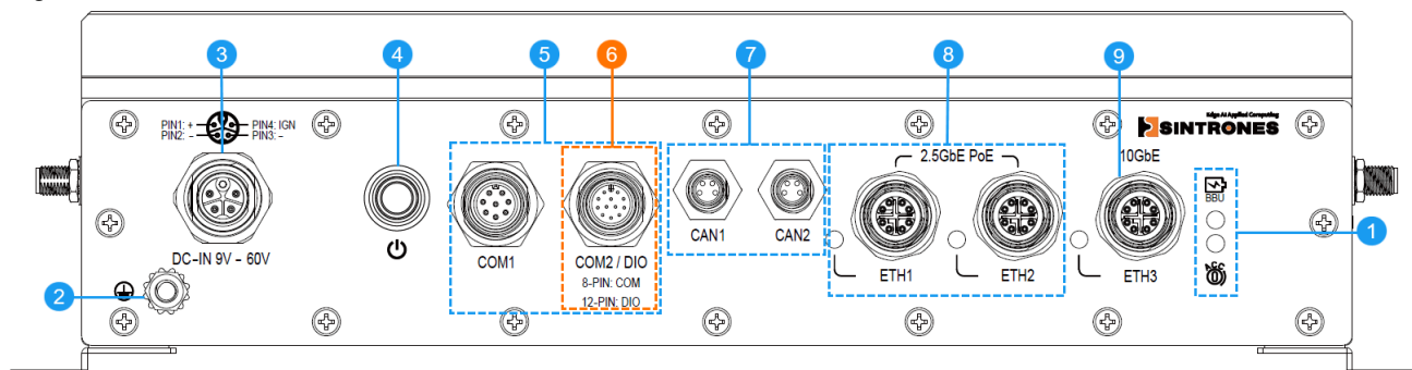
Figure 3-1 Front Panel of IBOX-650P-IP66-2S/-DIO
