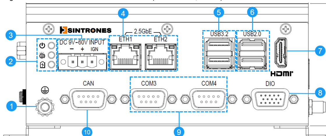
Figure 3-2 Front Panel of VBOX-3132-D25 (2 x 2.5 GbE, RJ-45)
