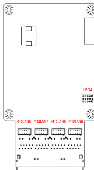
PoE Board (Bottom View) – PoE Models Only
