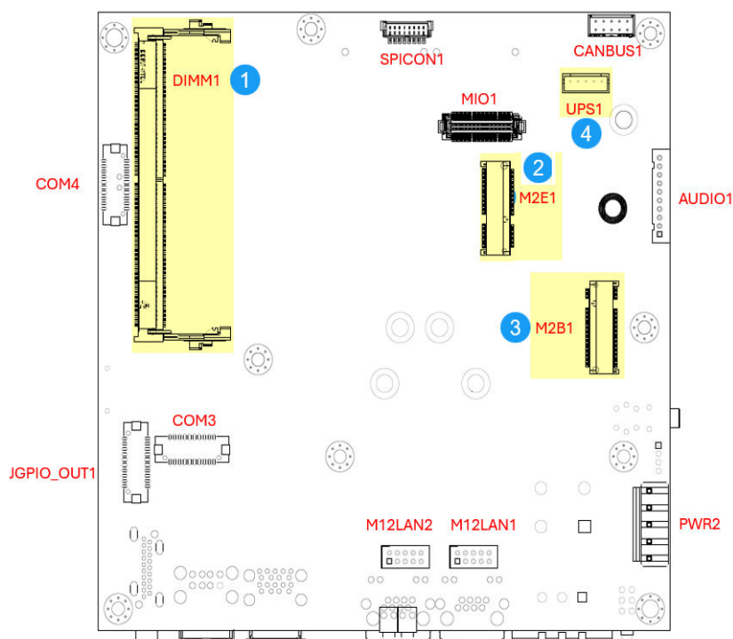
Mainboard of VBOX-3132 Series (Bottom View)
