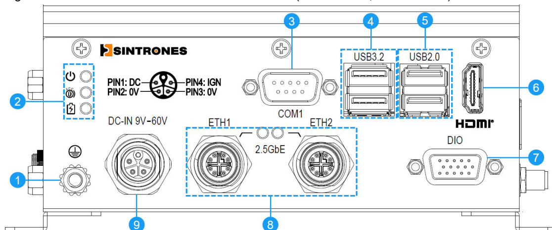
Figure 3-4 Front Panel of VBOX-3132-D25-M12X (2 x 2.5 GbE, M12 X-code)
