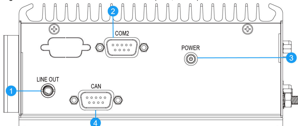
Figure 3-5 Left Side Panel of VBOX-3132P (PoE, RJ-45)
