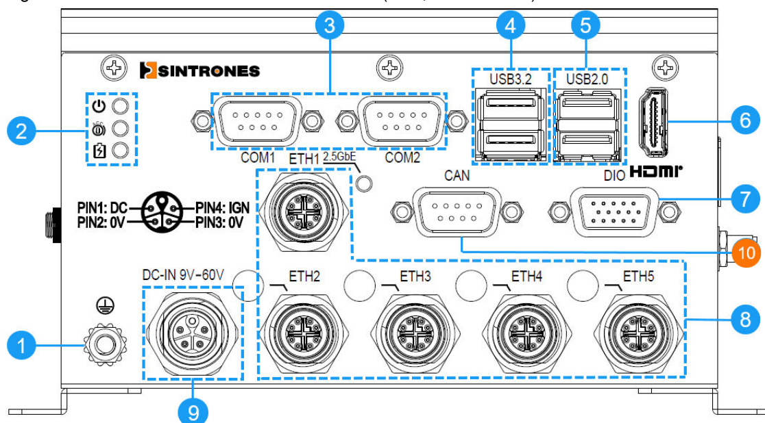
Figure 3-3 Front Panel of VBOX-3132P-M12X (PoE, M12 X-code)
