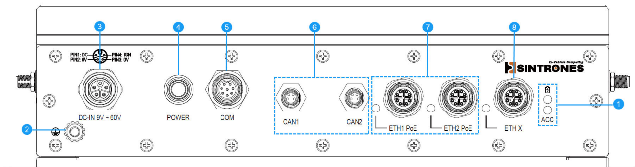
Figure 3-1 Front Panel of IBOX-650P-IP66
