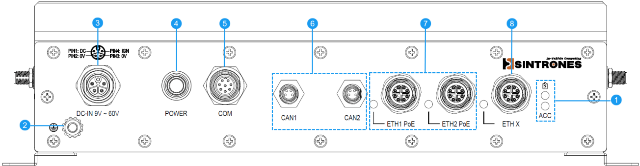
Figure 3-1 Front Panel of IBOX-650P-T1
